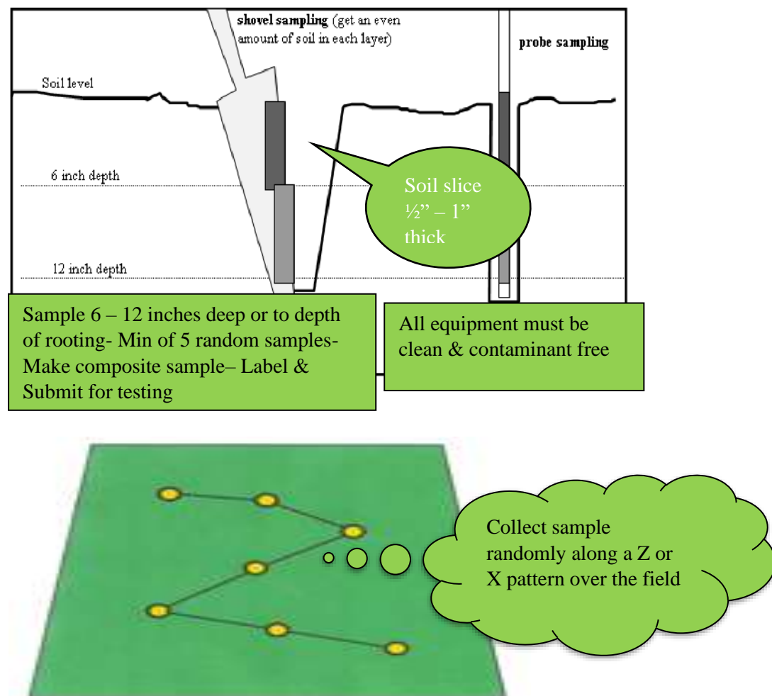
Figure 1: Soil testing illustration using shovel and soil probe. Location for sample collection
