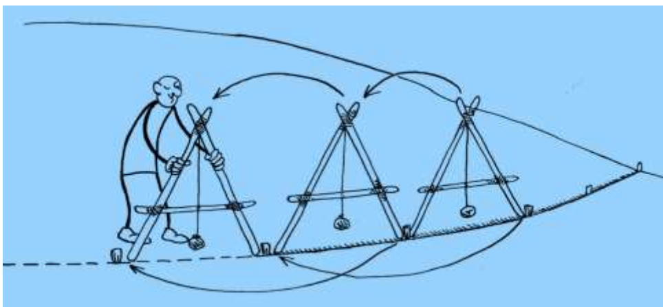
Figure 9: Using an A-frame level, finding and marking a level contour line
