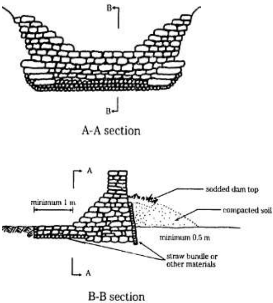
Figure 43: Masonry dam
