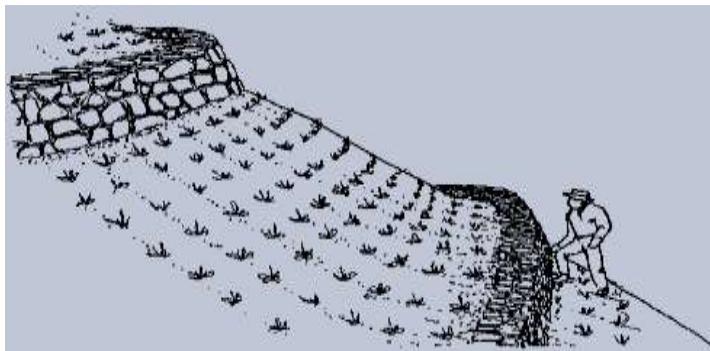
Figure 20: Stone wall or dead barriers installation
