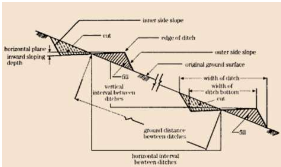
Figure 15: Cross-section of hillside ditch – Narrow and broad
