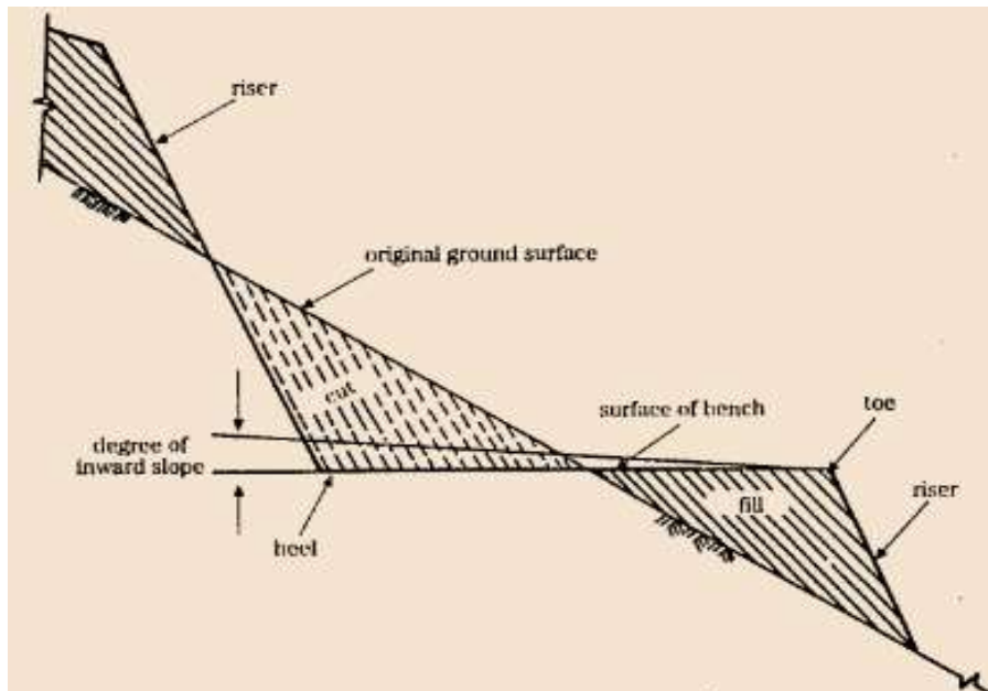
Figure 23: Reverse (inward) sloping bench terrace
