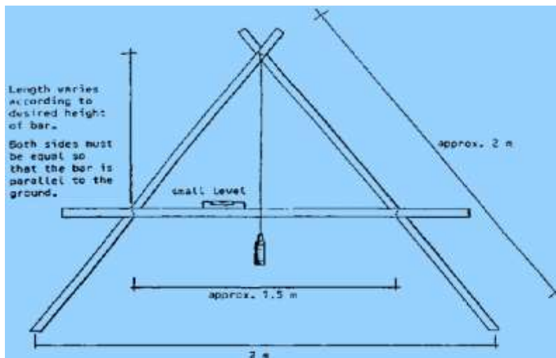
Figure 6: Calibrating the A-frame: steps one and two
