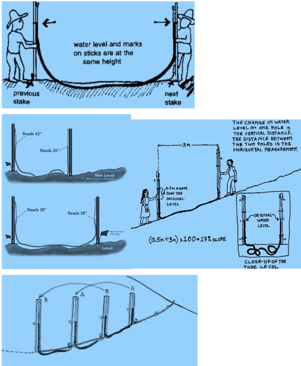
Figure 11: Hose level use illustration and calibration
