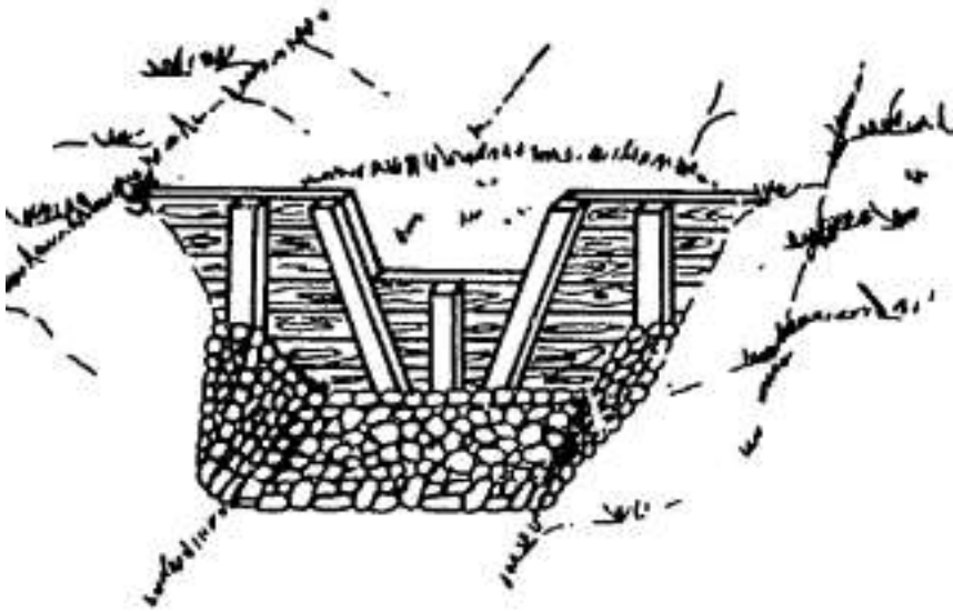
Figure 43: Masonry dam
