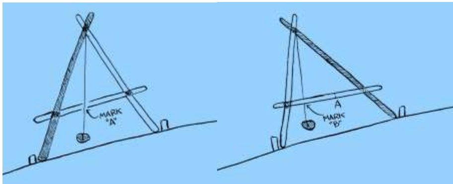
Figure 7: Calibrating the A-frame, final step
