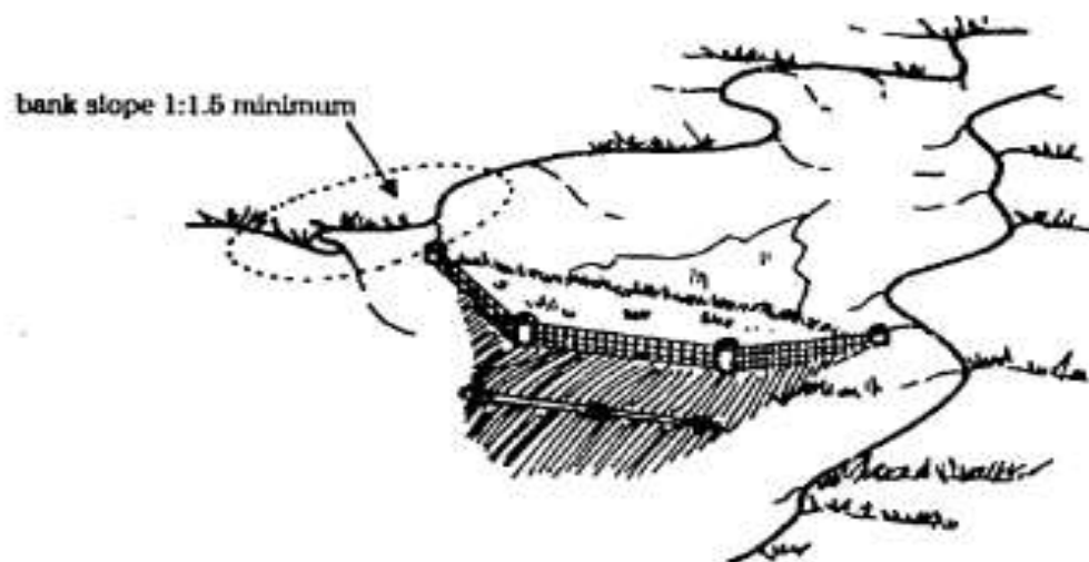
Figure 40: Timber dam
