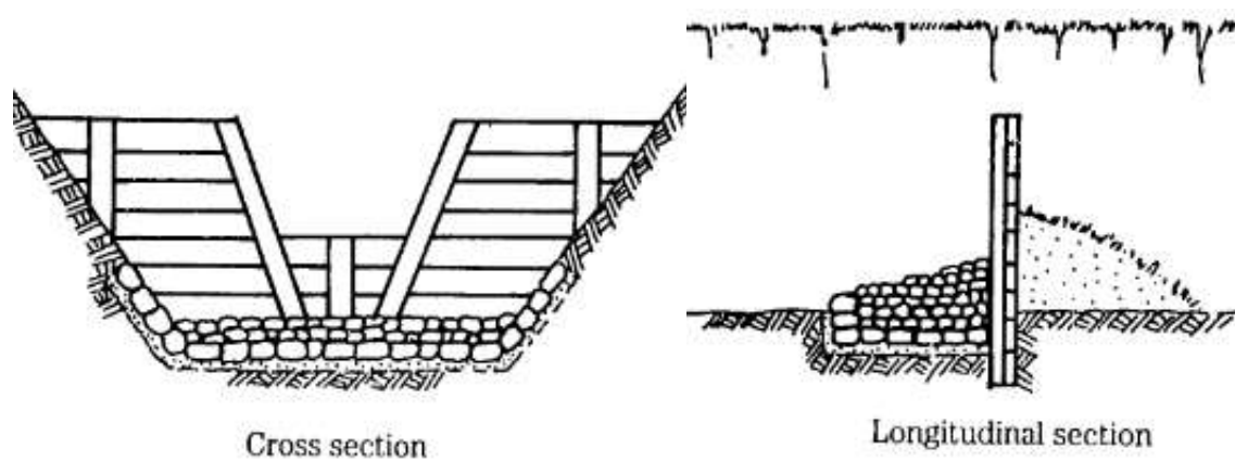
Figure 41: Plank dam
