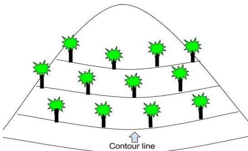
Figure 32: Topical view of design for contour planting
