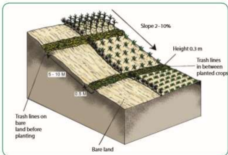
Figure 19: Replacement of decomposed trash lines
