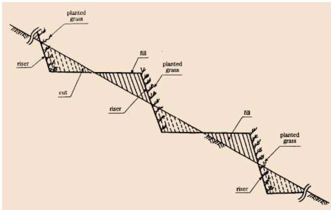
Figure 30: planted grass on risers of terrace
