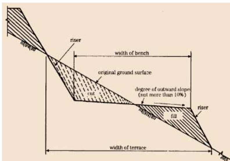
Figure 24: Outward sloping bench terrace
