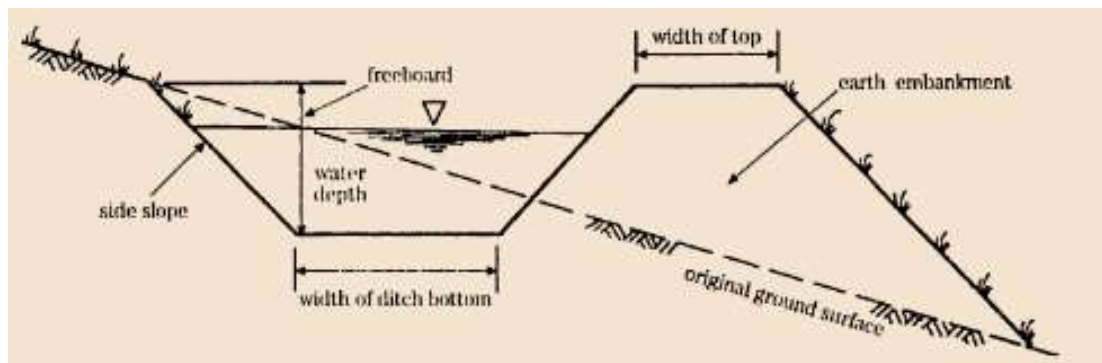
Figure 12: Illustration of diversion ditches
