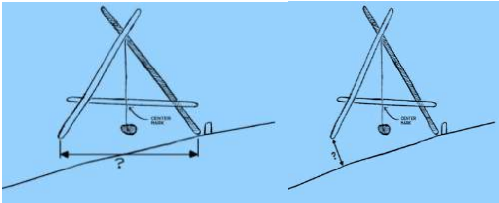
Figure 8: Using A-frame level to determine percent slope.
