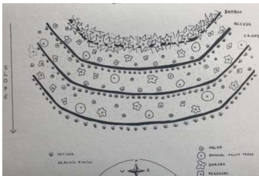
Figure 32: Topical view of design for contour planting
