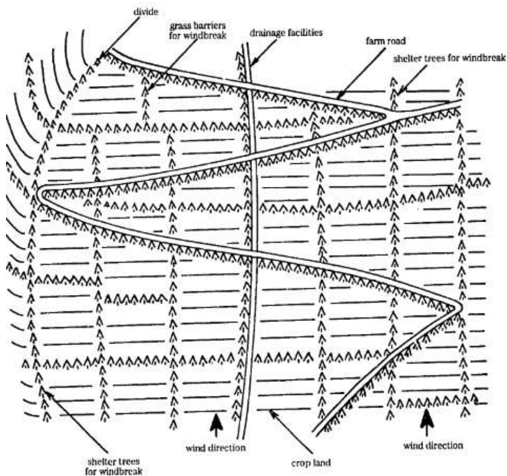
Figure 70: Typical on-farm wind break layout with other infrastructural features
