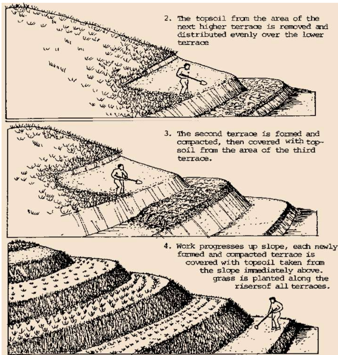
Figure 29: Bench terrace construction sequence "B"
