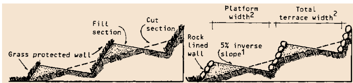
Figure 27: Continuous Bench terrace
