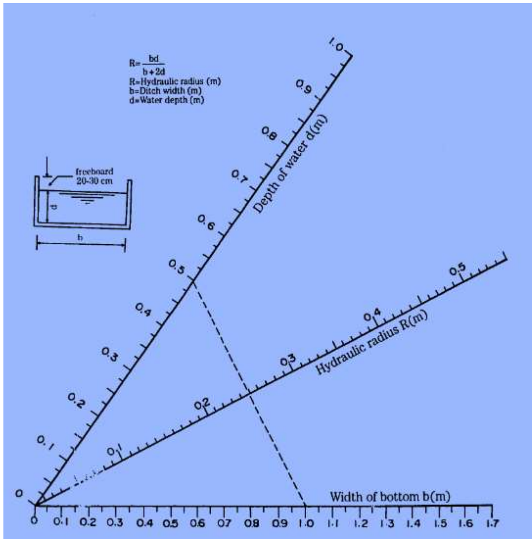
Figure 13: Estimation of Hydraulic radius of a diversion ditch with rectangular cross section nomograph
