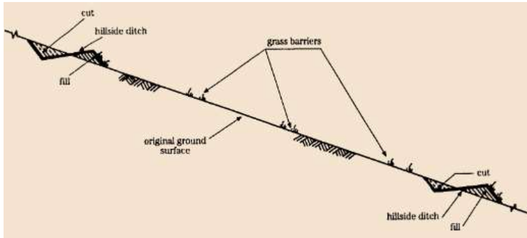
Figure 17: Illustration of Grass/live barriers
