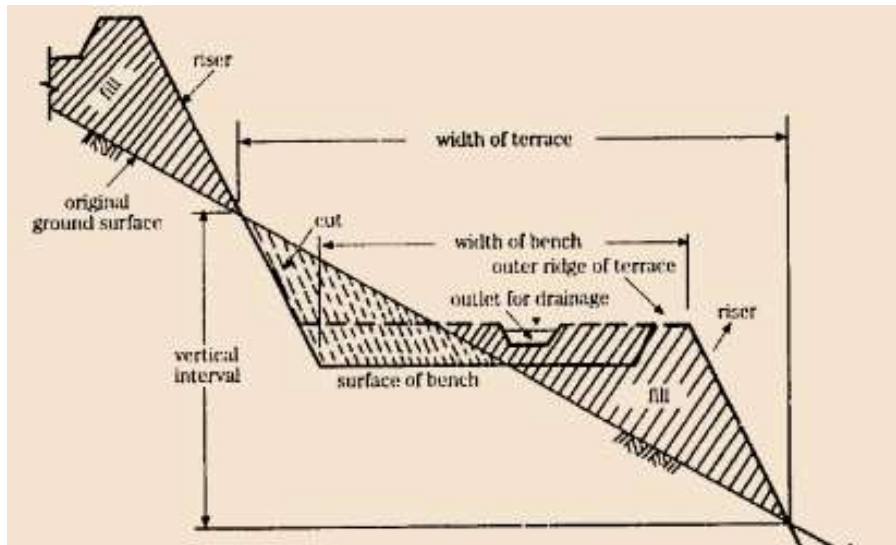
Figure 23: Reverse (inward) sloping bench terrace
